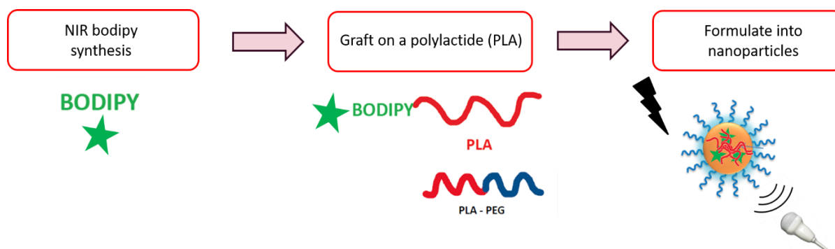
Figure 1 : From Bodipy to nanoparticles.
